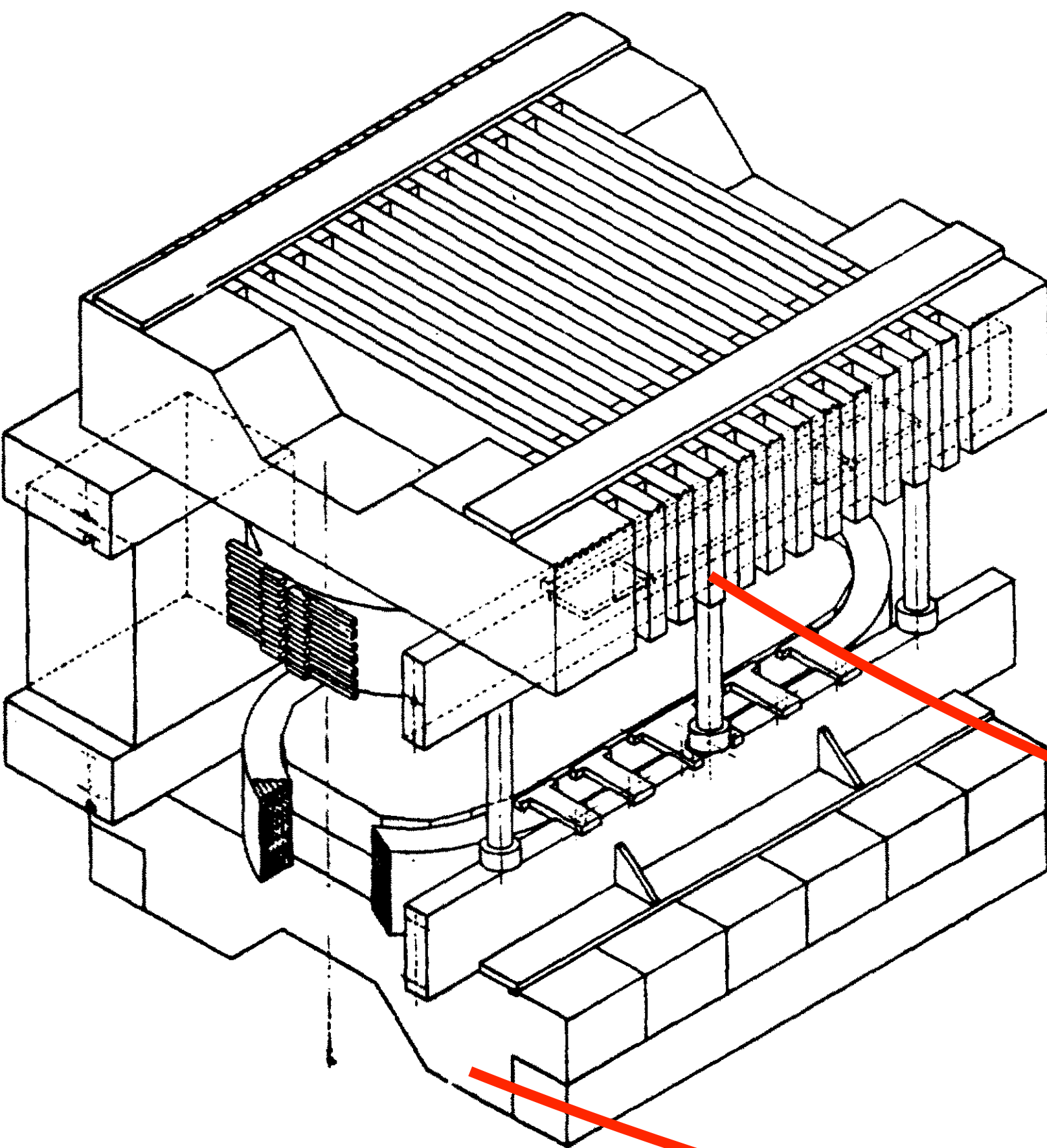
MPS magnet
